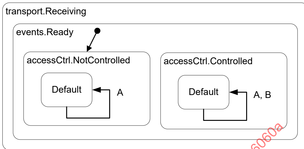
Figure 10 - RangeSensor service protocol behavior
