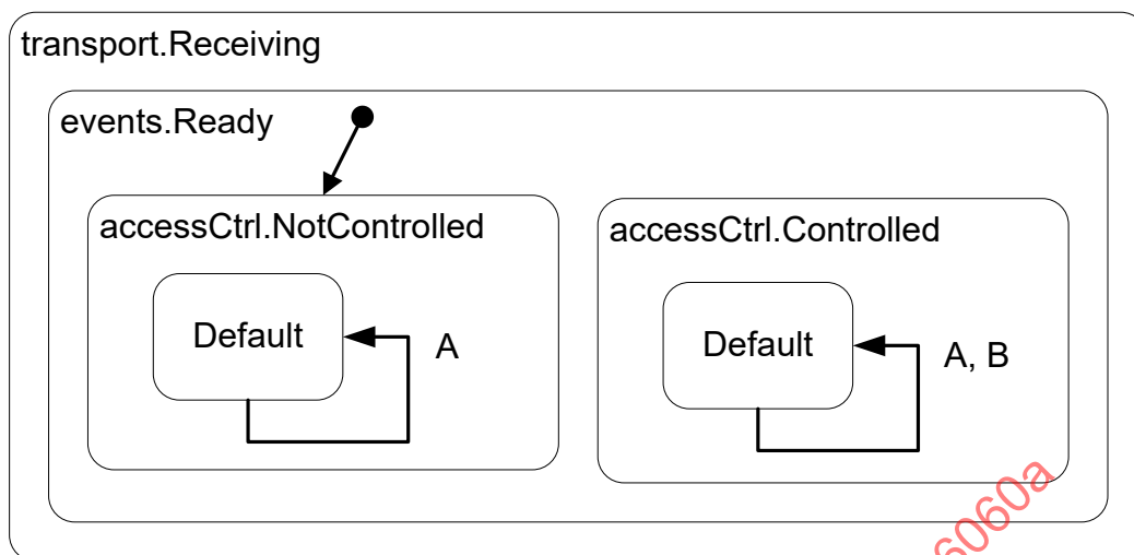
Figure 12 - Videolluminator service protocol behavior
