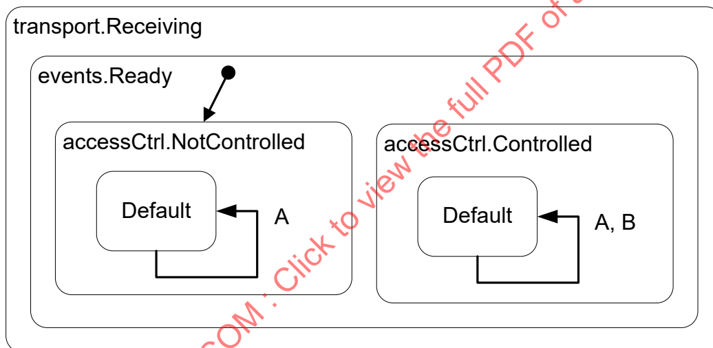
Figure 7 - H264VideoEncoding service protocol behavior
