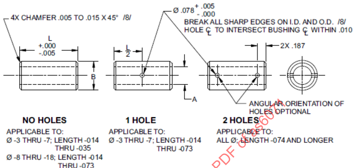
FIGURE 1 - AS6071 BUSHING
