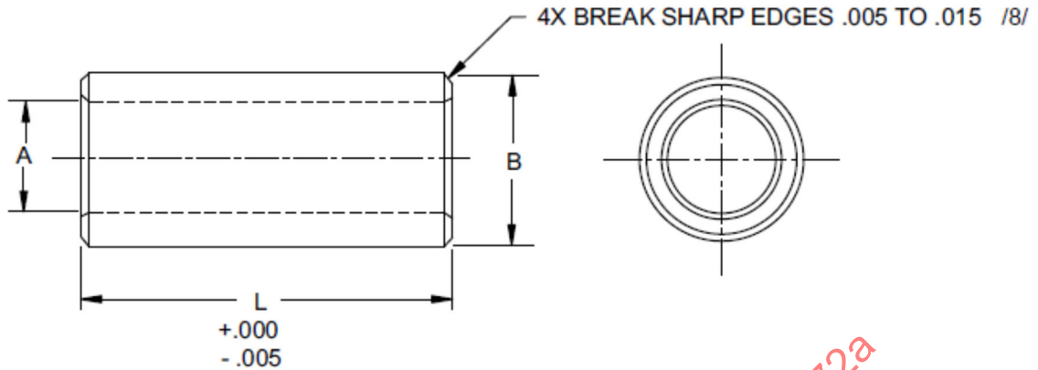
FIGURE 1 - AS6072 BUSHING
