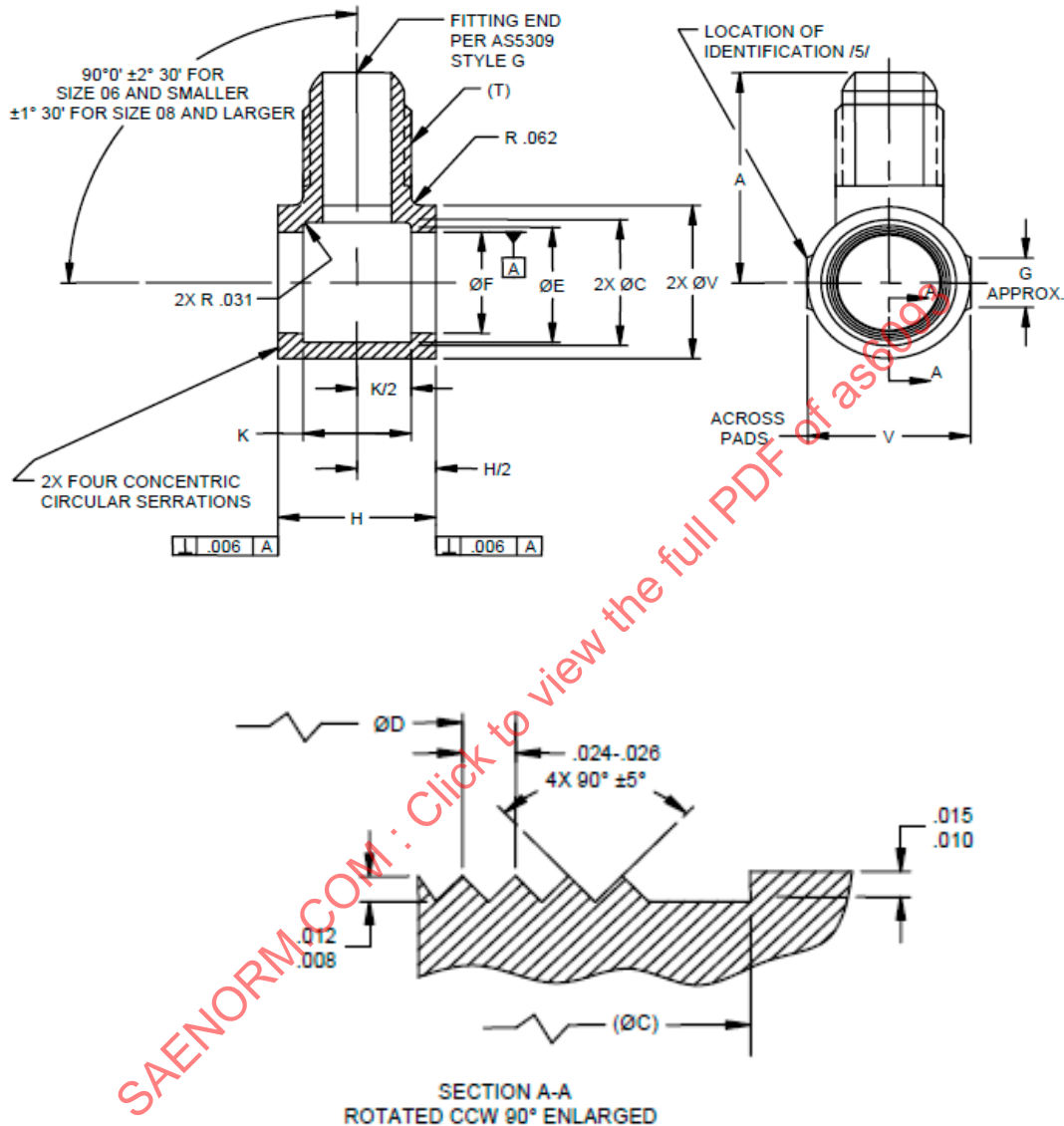
FIGURE 1 - FITTING, CONNECTOR, 90°
