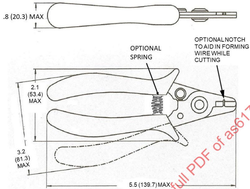
FIGURE 1 - BASIC WIRE CUTTER TOOL (INCHES)
