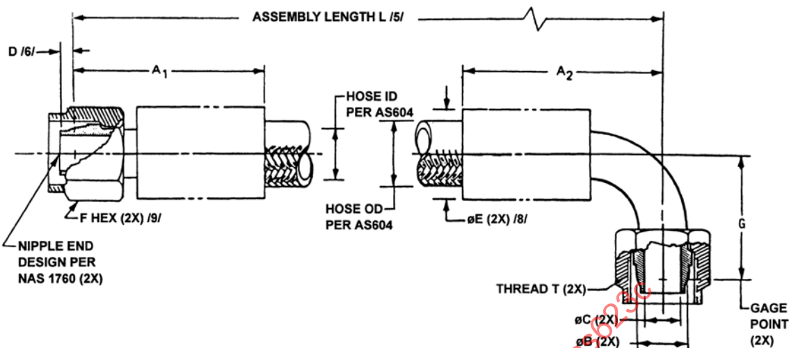
FIGURE 1 - HOSE AND FITTING DIMENSIONS
