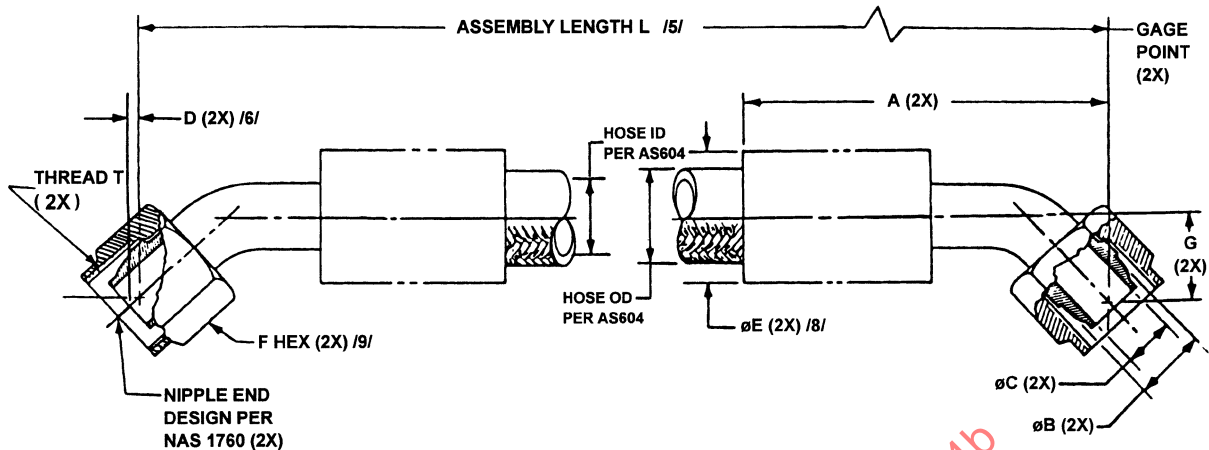
FIGURE 1 - HOSE AND FITTING DIMENSIONS
