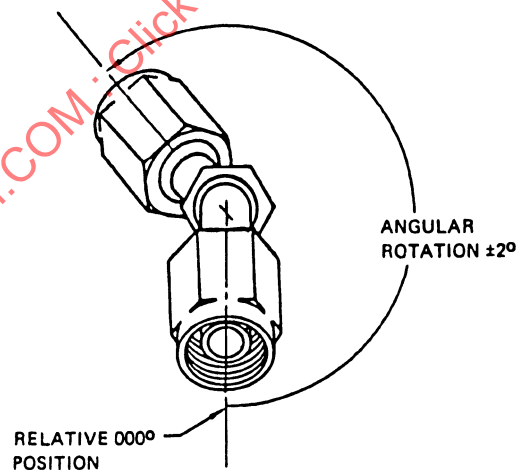
FIGURE 3 - FITTING ANGULAR ORIENTATION /19/
