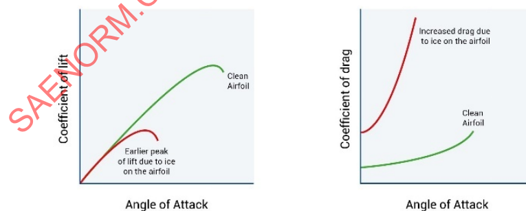
Figure A7 - Decrease in airfoil stall angle and increase in drag coefficient
