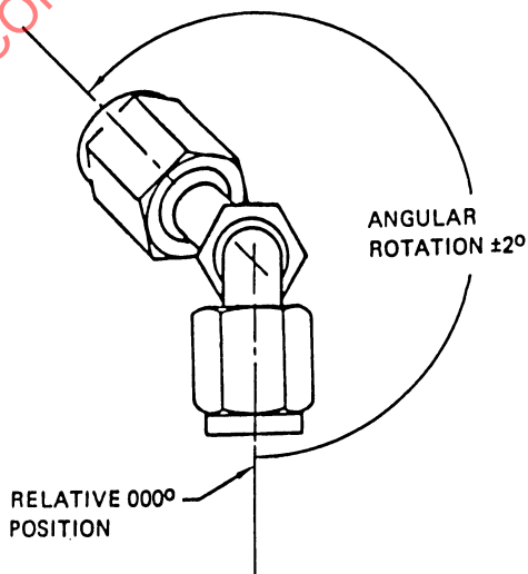
FIGURE 3 - FITTING ANGULAR ORIENTATION /18/
