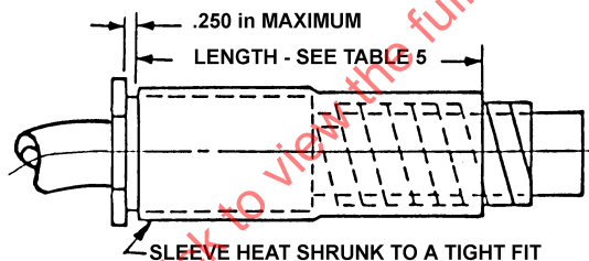
FIGURE 2 - TUBULAR/COIL ABRASION END /9/ /10/
