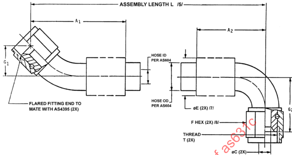
FIGURE 1 - HOSE AND FITTING DIMENSIONS
