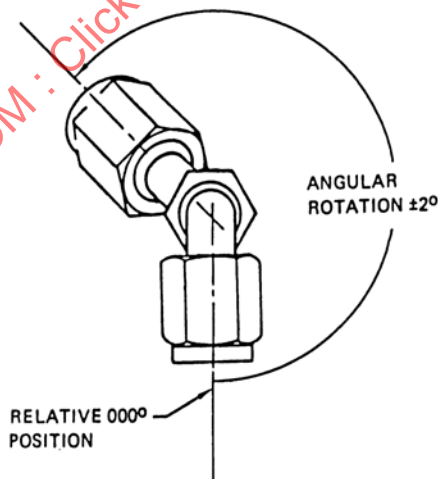
FIGURE 3 - FITTING ANGULAR ORIENTATION /18/
