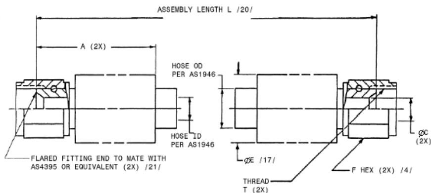
FIGURE 1 - HOSE ASSEMBLY
