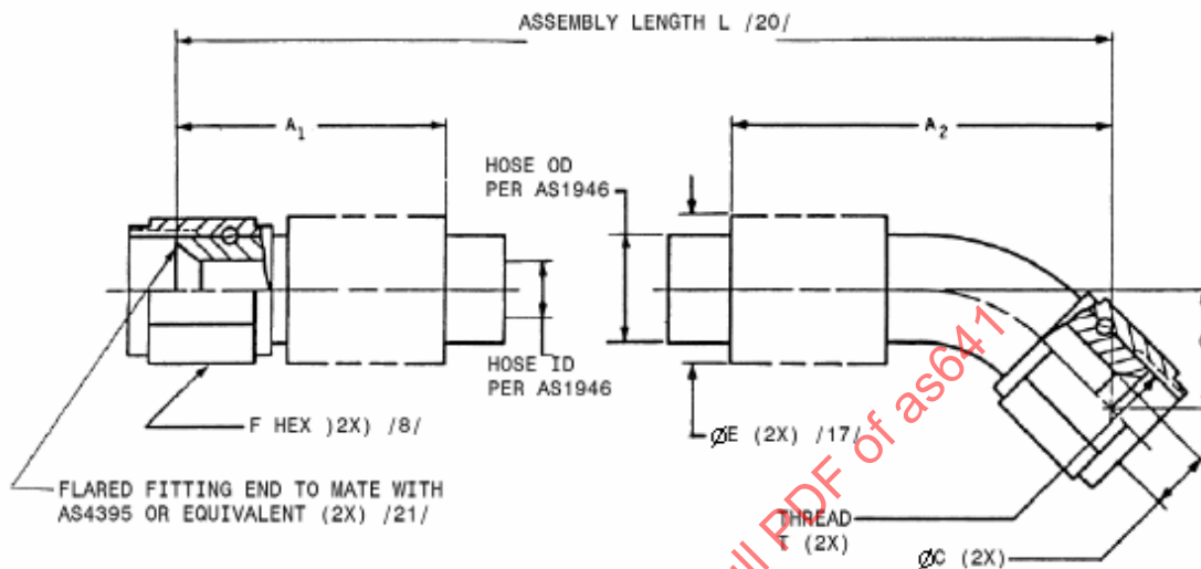
FIGURE 1 - HOSE ASSEMBLY
