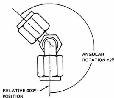
FIGURE 3 - FITTING ANGULAR ORIENTATION /26/
