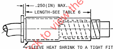
FIGURE 1 - HOSE ASSEMBLY
