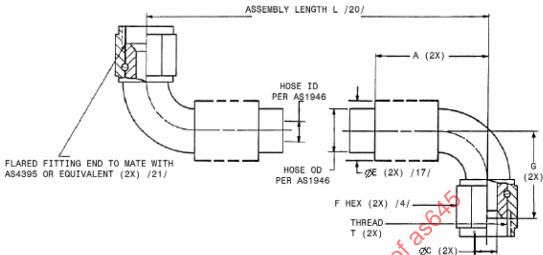
FIGURE 1 - HOSE ASSEMBLY
