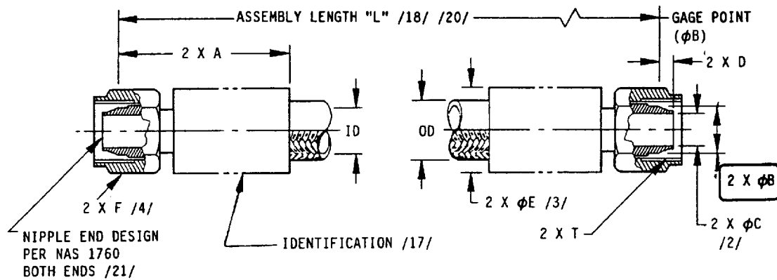
FIGURE 1 - HOSE ASSEMBLY
