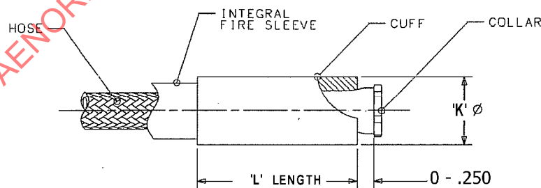
FIGURE 4 - SEE TABLE 8 /27/
