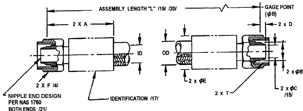
FIGURE 1 - HOSE ASSEMBLY
