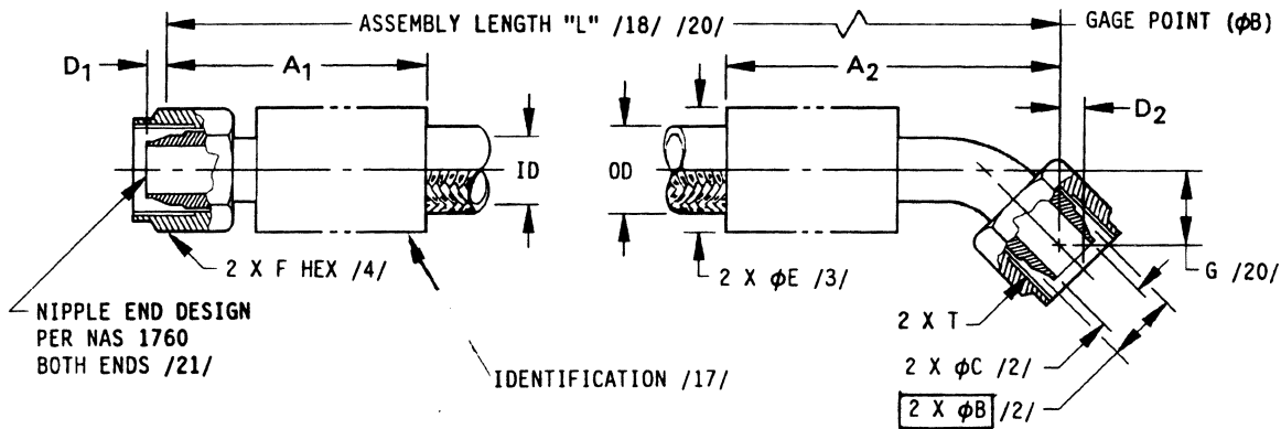
FIGURE 1 - HOSE ASSEMBLY
