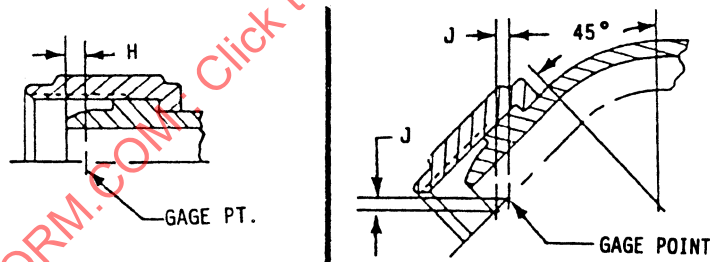
FIGURE 3 - SEE TABLE 7
