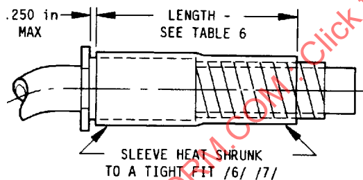
FIGURE 2 - ABRASION SLEEVE ATTACHMENT
