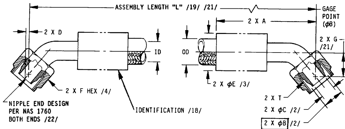
FIGURE 1 - HOSE ASSEMBLY
