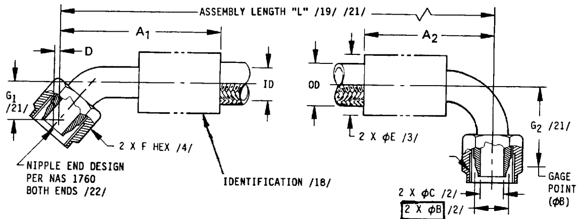
FIGURE 1 - HOSE ASSEMBLY
