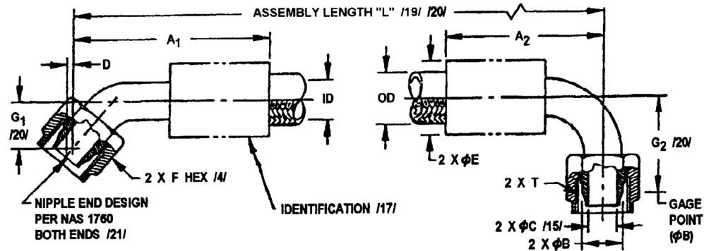
FIGURE 1 - HOSE ASSEMBLY
