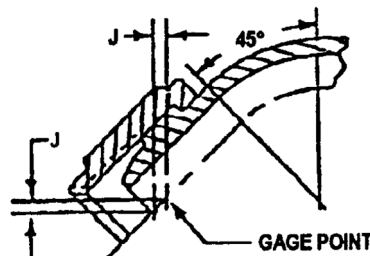
FIGURE 3 - FITTING ANGULAR POSITION /26/
