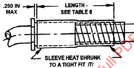
FIGURE 2 - ABRASION SLEEVE ATTACHMENT
