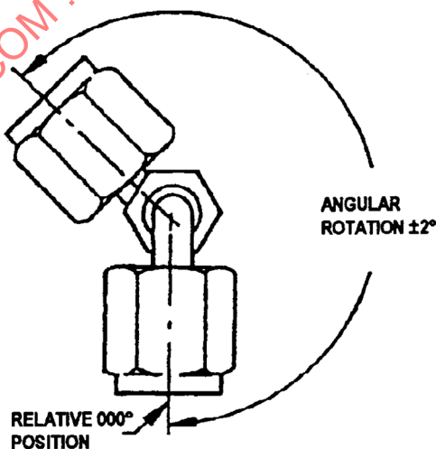
FIGURE 3 - FITTING ANGULAR POSITION (26/)
