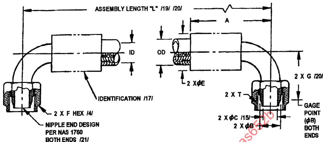
FIGURE 1 - HOSE ASSEMBLY
