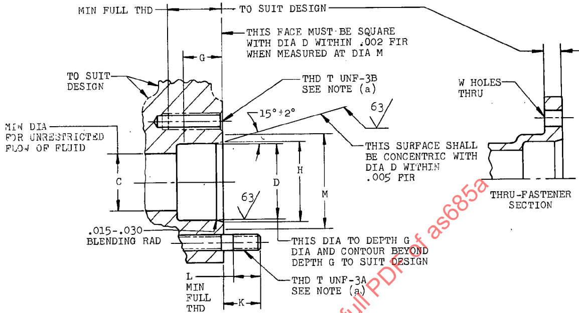
SECTION X-X (Typical)
