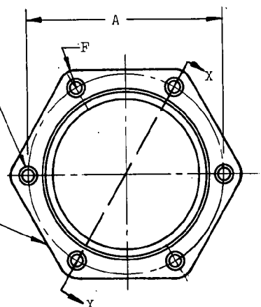
MOUNTING PAD FOR FITTINGS SIZES -40 THRU -64
