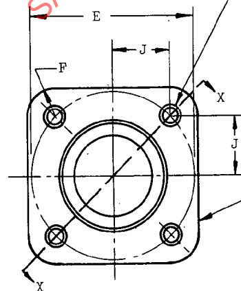
MOUNTING PAD FOR FITTINGS SIZES -12 THRU -32
