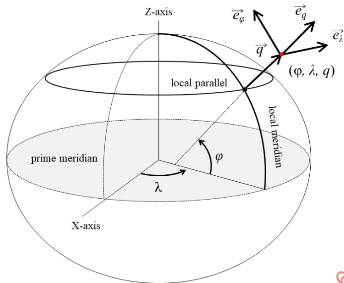
Figure 25 - WGS84 Ellipsoidal coordinate system (Euclidean space)
