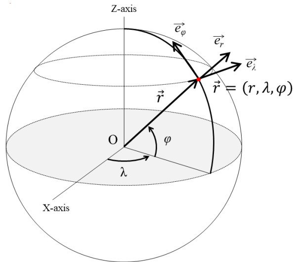
Figure 23 - SphericalRAE coordinate system (Euclidean space)
