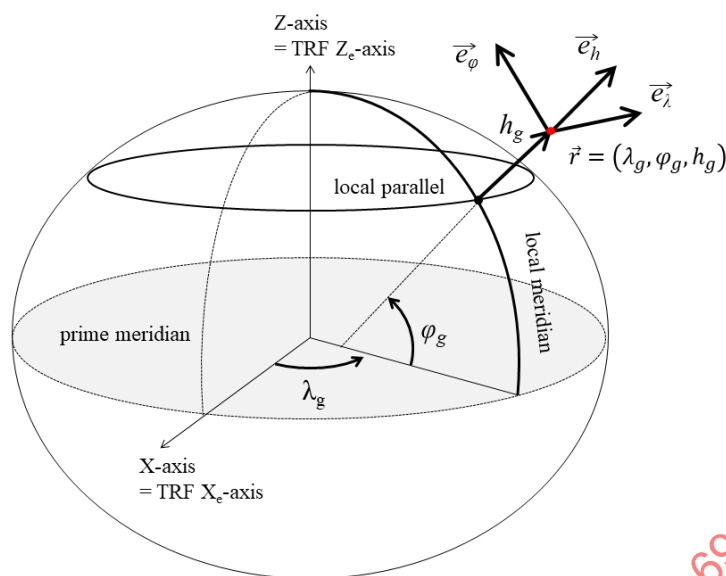
Figure 15 - Vehicle-carried LTP coordinate datum
