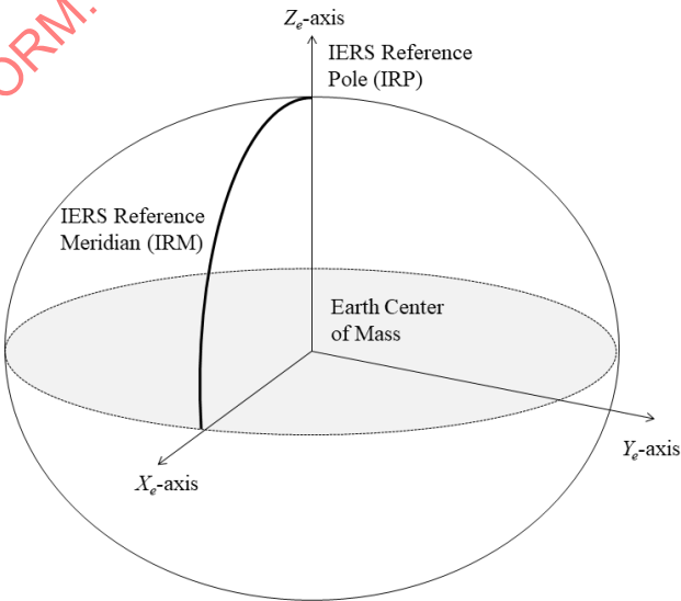
Figure 8 - WGS 84 reference frame
