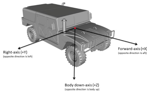
Figure 12 - Vehicle body CD applied to wheeled vehicle
