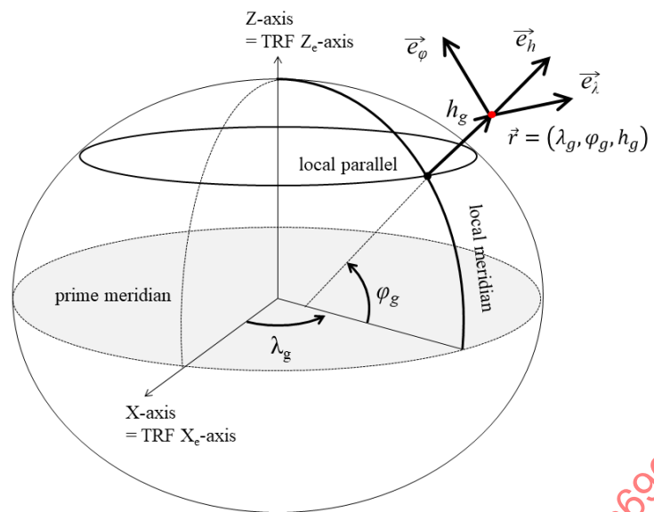
Figure 14 - Vehicle-carried LTP coordinate datum
