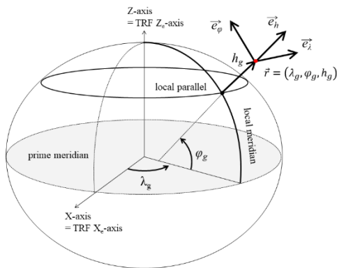
Figure 13 - Earth-fixed LTP coordinate datum
