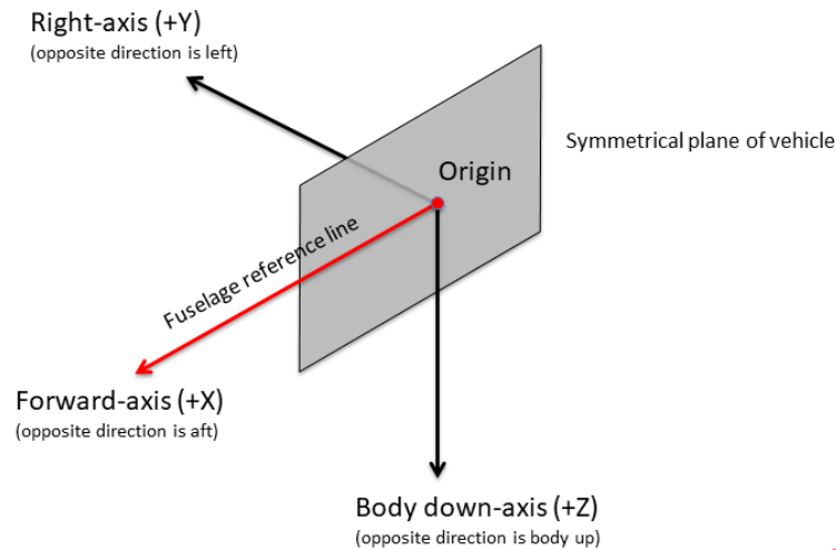
Figure 9 - Vehicle body coordinate datum
