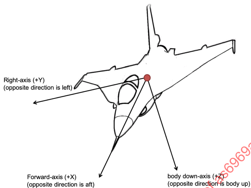
Figure 6 - Vehicle body CD applied to aircraft
