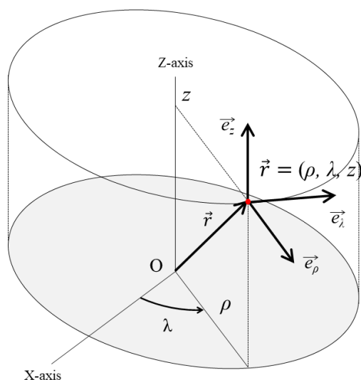
Figure 19 - Cylindrical coordinate system (Euclidean space)
