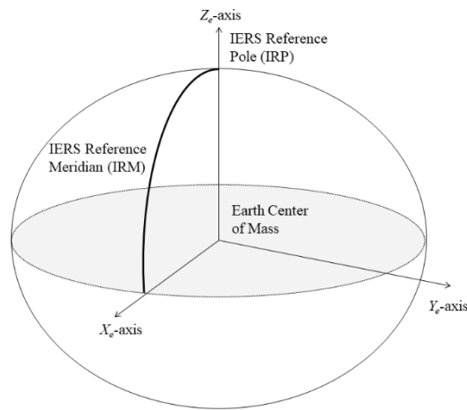
Figure 2 - WGS 84 CTRS
