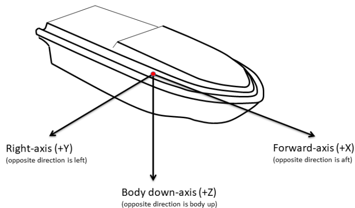
Figure 11 - Vehicle body CD applied to vessel (i.e., boat or ship)
