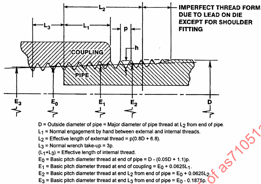
FIGURE 2 - AERONAUTICAL NATIONAL TAPER PIPE THREAD DIMENSIONS
