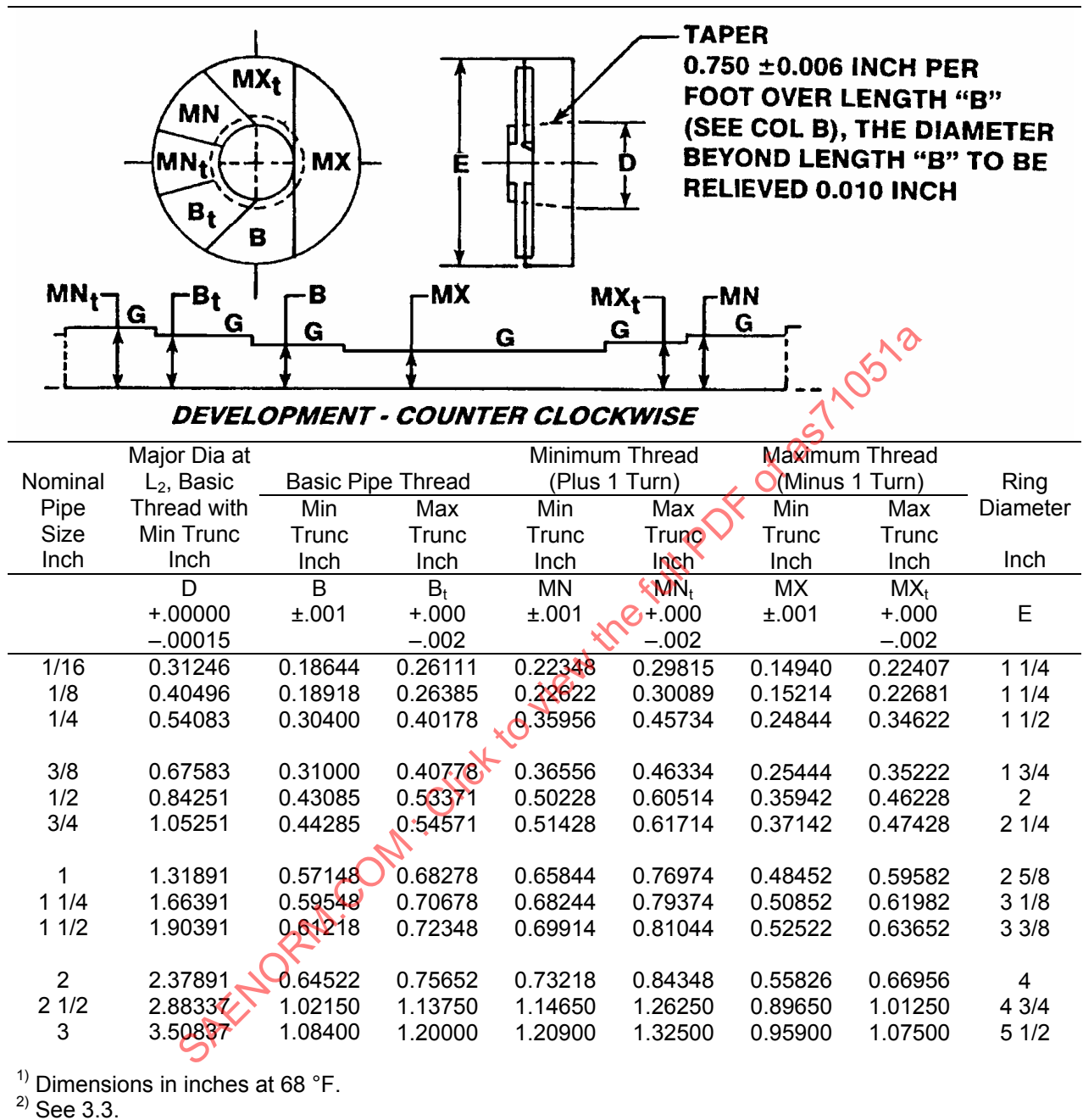
FIGURE 5 - PLAIN TAPER RING GAGE
