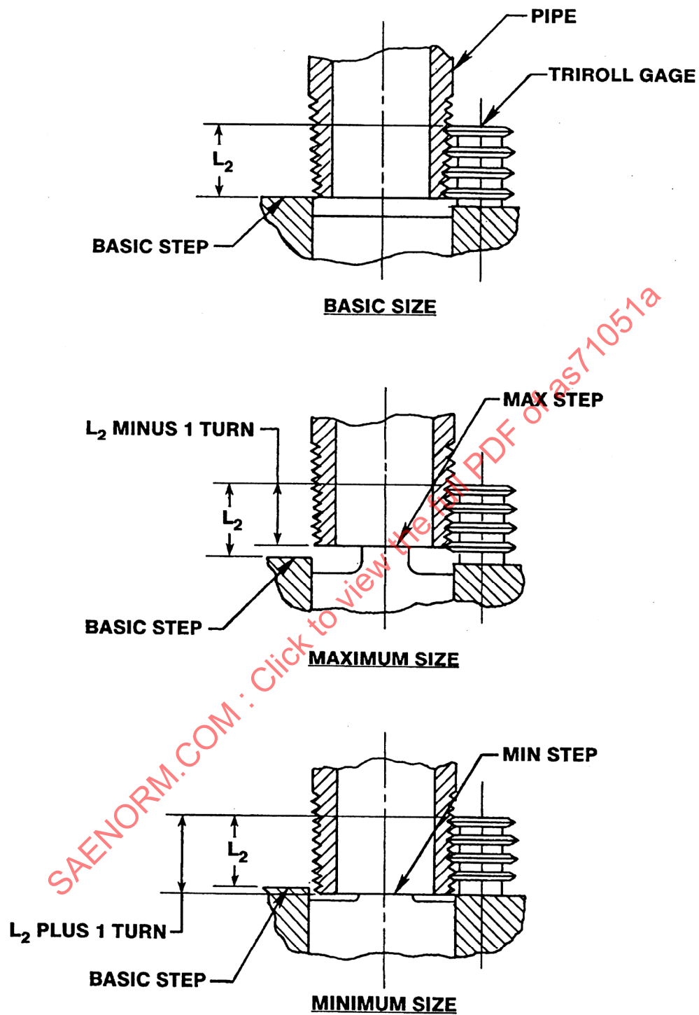
FIGURE 7 - APPLICATION OF TRIROLL GAGE
