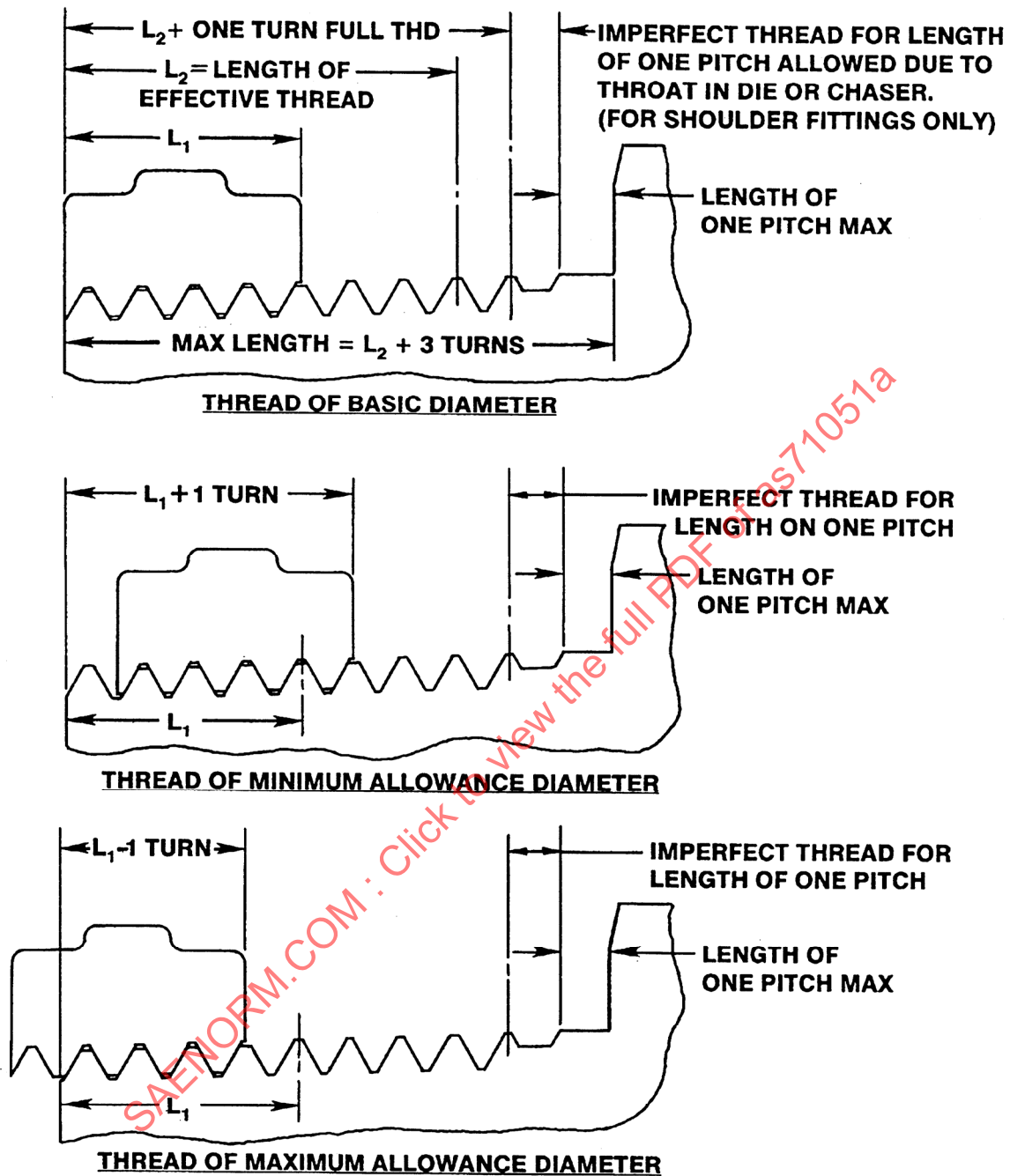
FIGURE 9 - APPLICATION OF THIN RING TAPER THREAD GAGE (0.15P)
