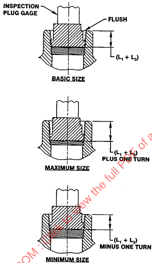
FIGURE 11 - APPLICATION OF L_3 TAPER THREAD PLUG GAGE
