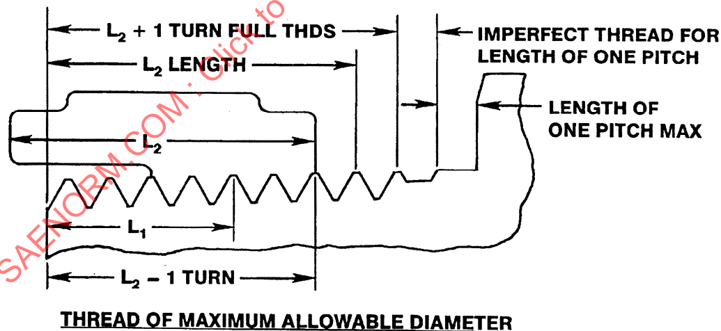
FIGURE 8 - APPLICATION OF FULL RING TAPER THREAD GAGE
