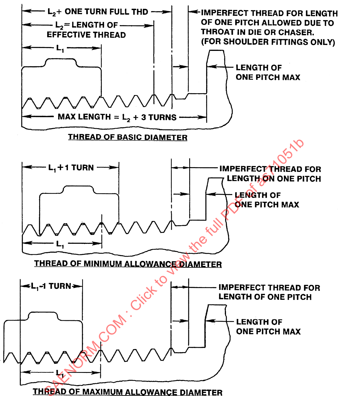
FIGURE 9 - APPLICATION OF THIN RING TAPER THREAD GAGE (.15P)
