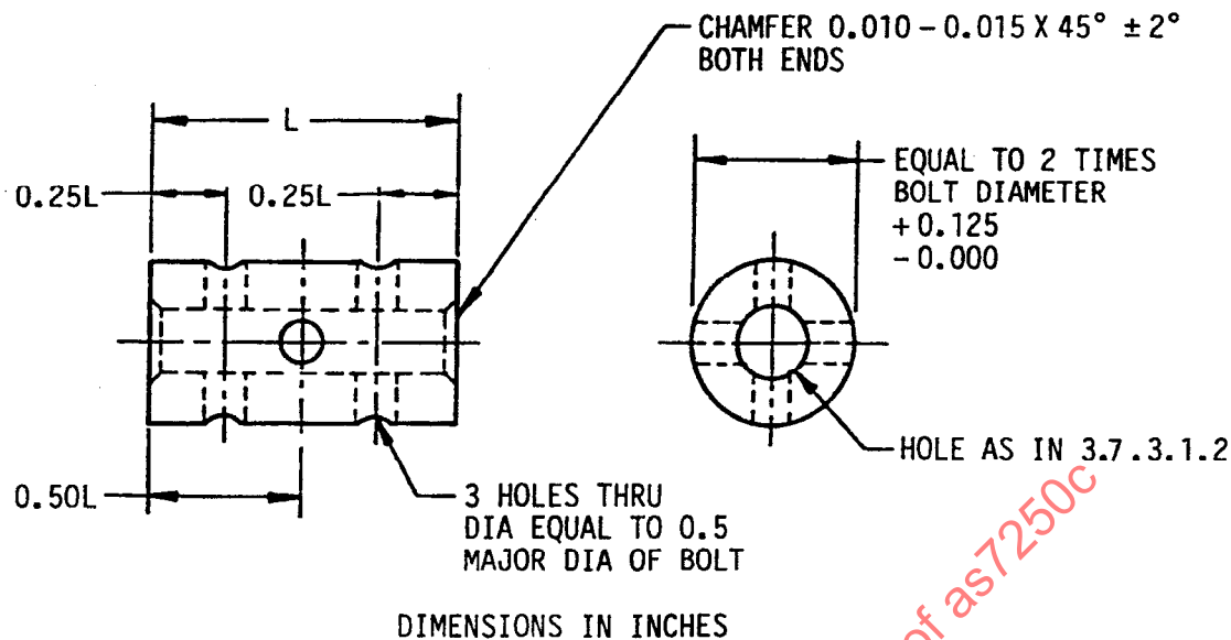
FIGURE 2 - SPACER-TYPE FIXTURE
