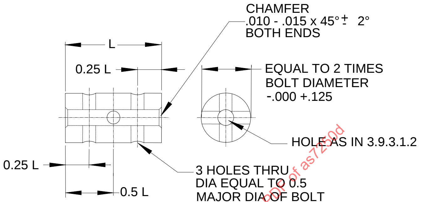
FIGURE 2 - SPACER-TYPE FIXTURE
