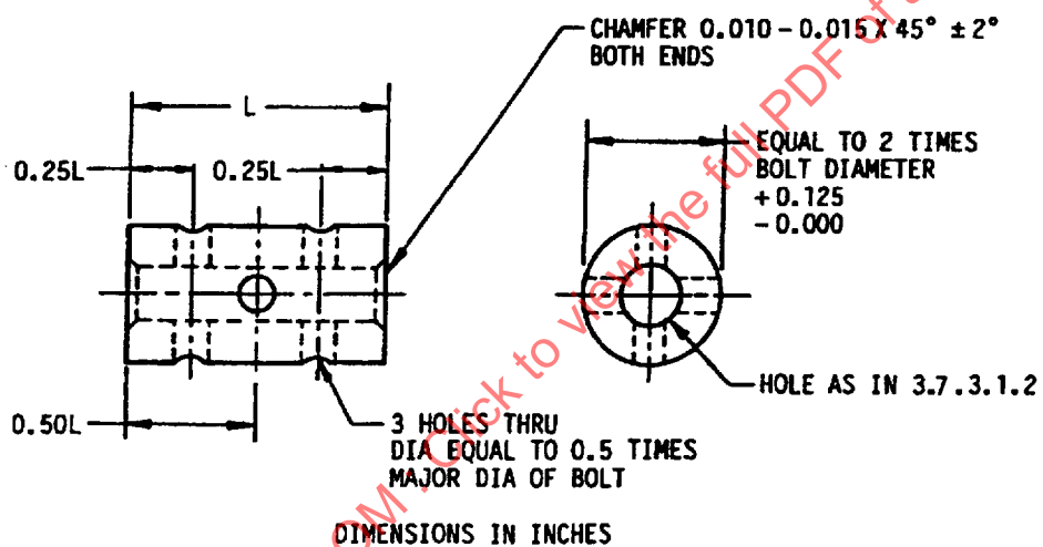
FIGURE 2 - Spacer-Type Fixture
