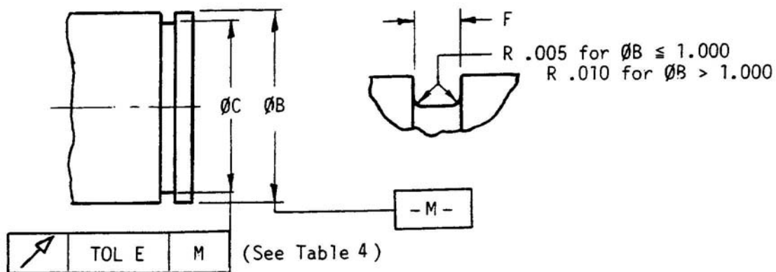
FIGURE 1 - Groove Dimensions, Type I, Classes 1 and 2 Retaining Rings (See Table 5)
