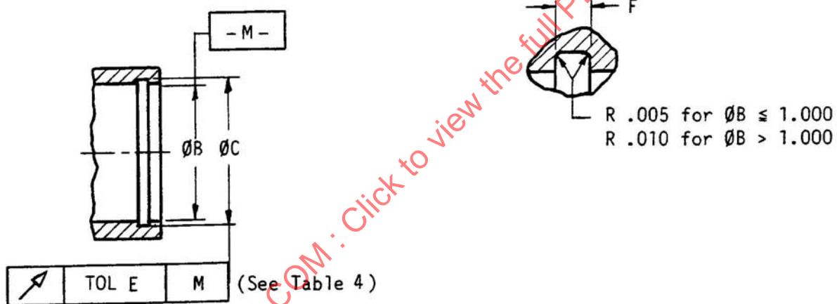
FIGURE 2 - Groove Dimensions, Type II, Classes 1 and 2 Retaining Rings (See Table 6)
