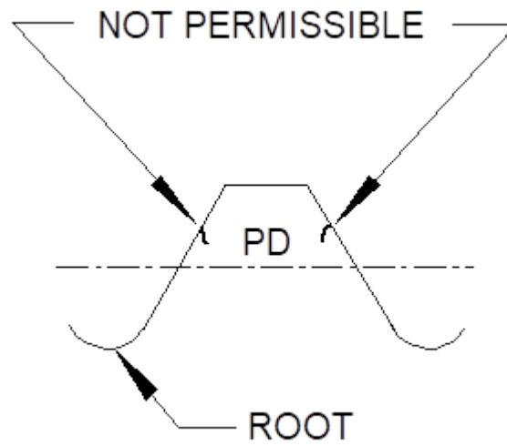
Figure 5 - Laps above PD extending toward root, rolled thread
