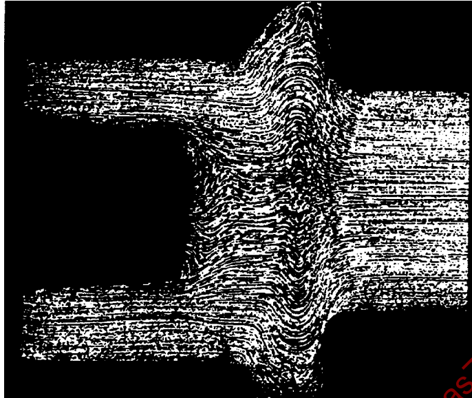
FIGURE 1B - MINIMUM ACCEPTABLE STANDARD SHOWING MAXIMUM PERMISSIBLE CUTTING OF GRAIN FLOW AFTER MACHINING TO REMOVE CONTAMINATION OXIDE.
