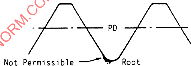
Figure 3 - Root defects, rolled thread
