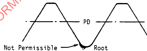
FIGURE 3 - ROOT DEFECTS, ROLLED THREAD
