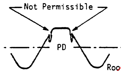
FIGURE 5 - LAPS ABOVE PD EXTENDING TOWARD ROOT, ROLLED THREAD
