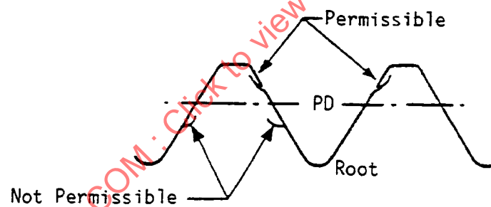
FIGURE 6 - LAPS EXTENDING TOWARDS CREST, ROLLED THREAD
