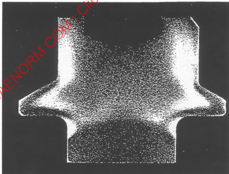
FIGURE 1A - SATISFACTORY HEAT PATTERN, HEADED BLANK, BEFORE HEAT TREATMENT
