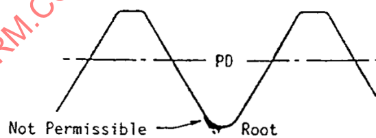
FIGURE 4 - ROOT DEFECTS, ROLLED THREAD
