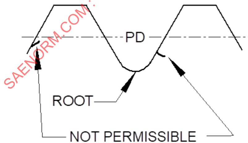
Figure 6 - Laps extending towards crest, rolled thread
