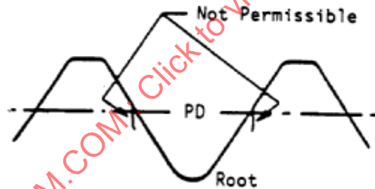
FIGURE 5 - Laps Below PD Extending Toward Root, Rolled Thread
