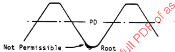
FIGURE 4 - Root Defects, Rolled Thread
