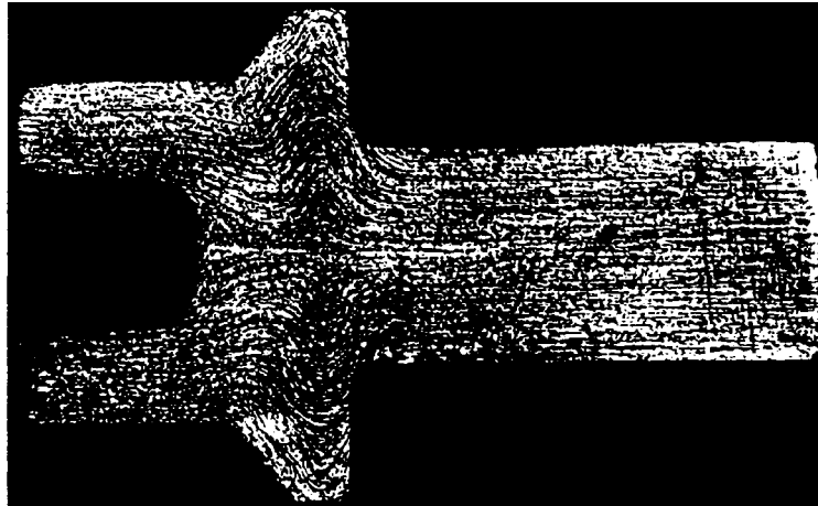
FIGURE 1C - UNACCEPTABLE GRAIN FLOW
