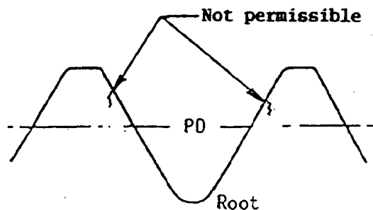
(R) FIGURE 6 - Laps Above PD Extending Toward Root, Rolled Thread
