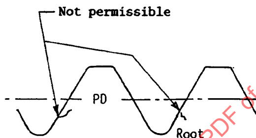
(R) FIGURE 7 - Laps Below PD Extending in Any Direction, Rolled Thread
