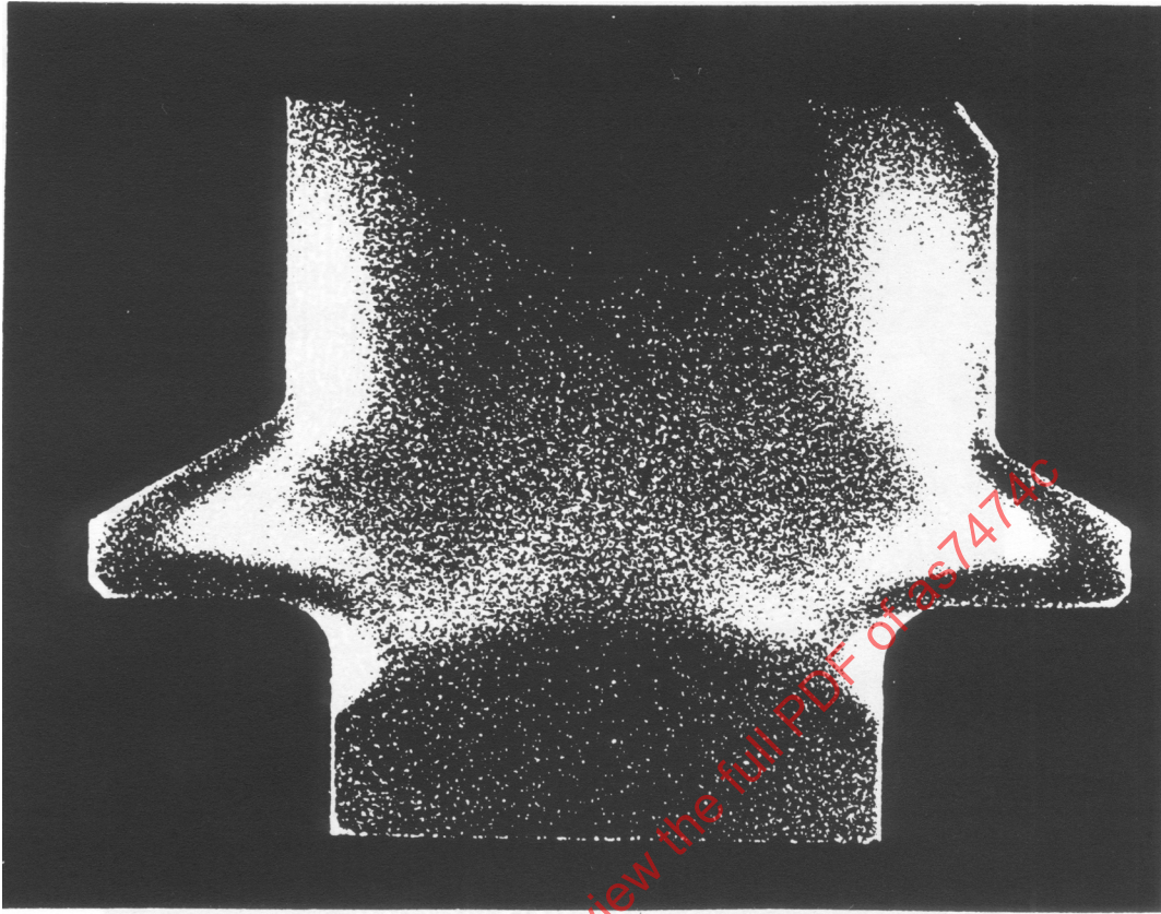
FIGURE 1A - HEAD-TO-SHANK SECTION THROUGH FINISHED PART SHOWS EVIDENCE THAT HEAD WAS FORMED BY FORGING.
