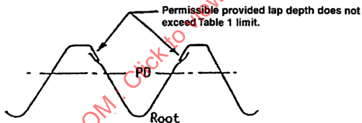
(R) FIGURE 5 - Laps Above Pitch Diameter Extending Towards Crest, Rolled Thread
