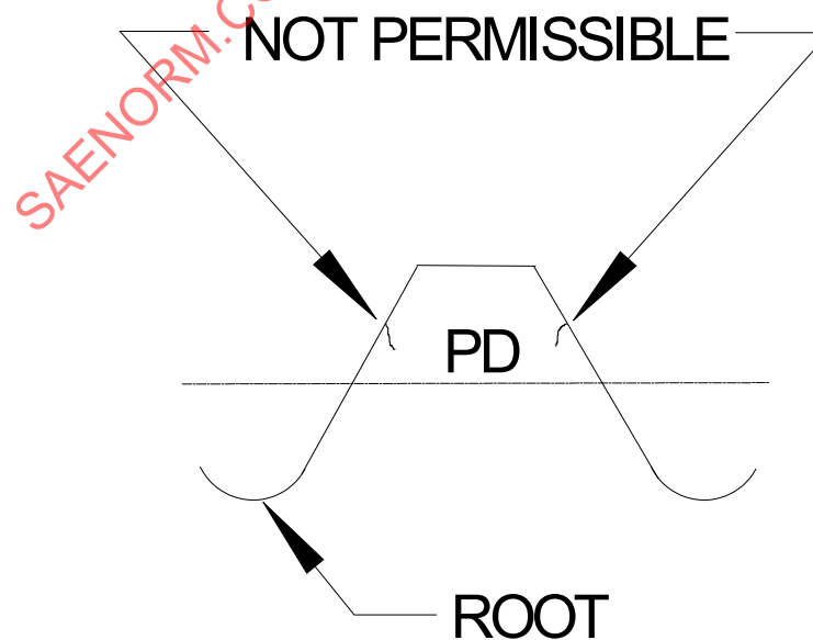
Figure 5 - Laps above PD extending toward root, rolled thread
