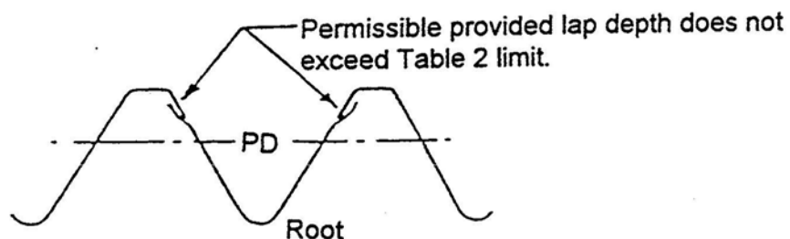
FIGURE 5 - LAPS ABOVE PITCH DIAMETER EXTENDING TOWARDS CREST, ROLLED THREAD
