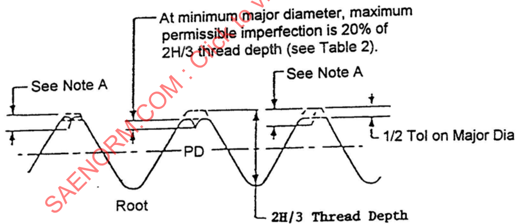
FIGURE 8 - CREST CRATERS AND CREST LAPS, ROLLED THREAD
