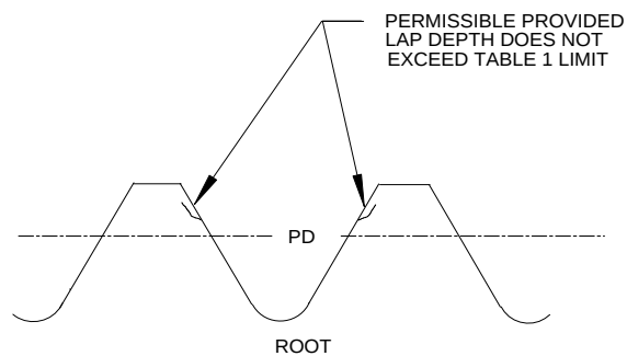
FIGURE 5 - LAPS ABOVE PITCH DIAMETER EXTENDING TOWARDS CREST, ROLLED THREAD
