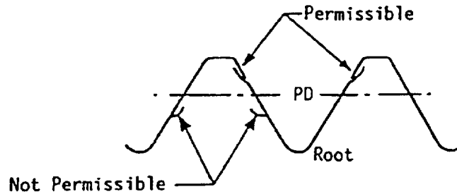
FIGURE 5 - Laps Extending Towards Crest, Rolled Thread
