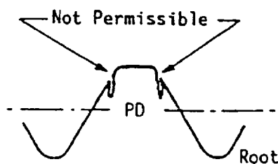
FIGURE 4 - Laps Above PD Extending Toward Root, Rolled Thread
