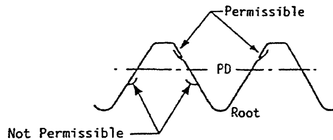
FIGURE 5 - Laps Extending Towards Crest, Rolled Thread
