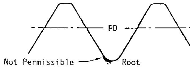
FIGURE 2 - ROOT DEFECTS, ROLLED THREAD
