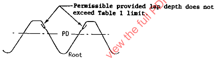
FIGURE 3 - LAPS ABOVE PITCH DIAMETER EXTENDING TOWARDS CREST, ROLLED THREAD
