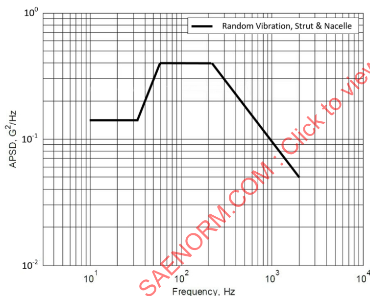
Figure 33 - High energy random vibration spectra
