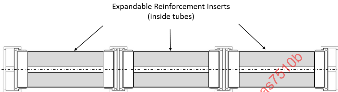
Figure 25 - Dynamic shear test reinforcement insert placement (optional)
