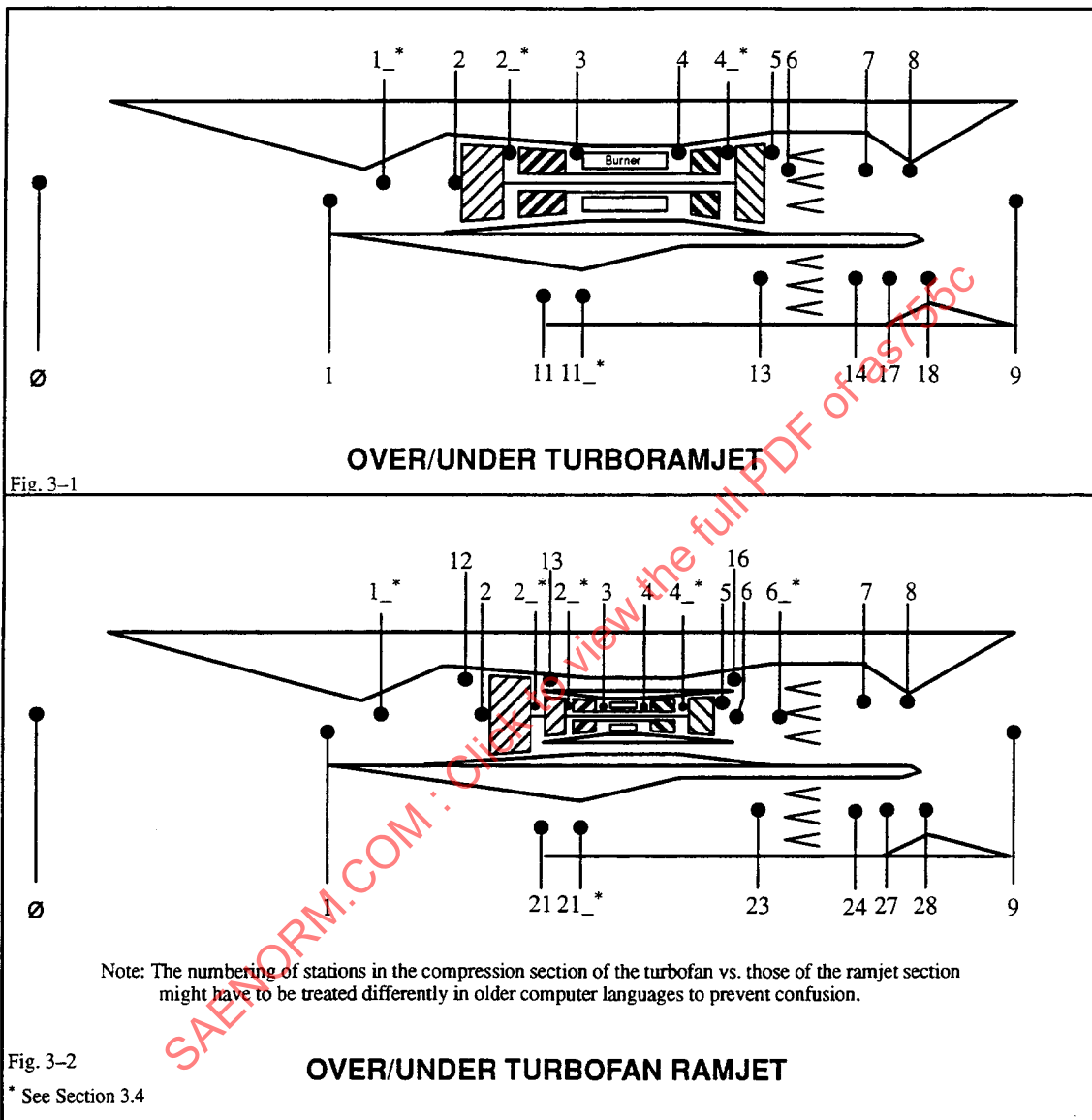
FIGURE 3 - Examples of Station Designation for Other Airbreathing Propulsion Systems (Reference Section 3)
