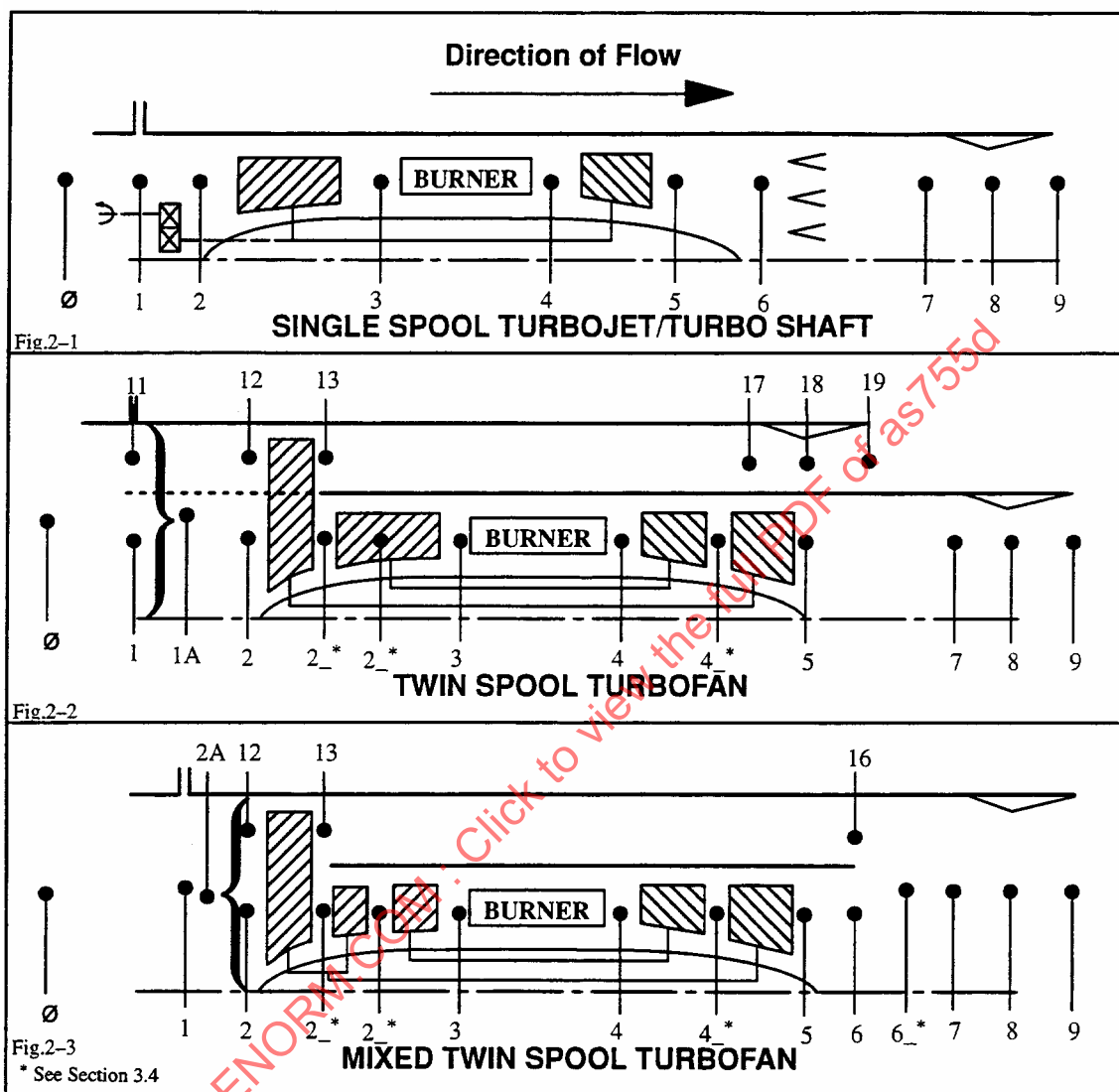
FIGURE 2 - Examples of Station Designation for Gas Turbine Engines (Reference Section 3)
