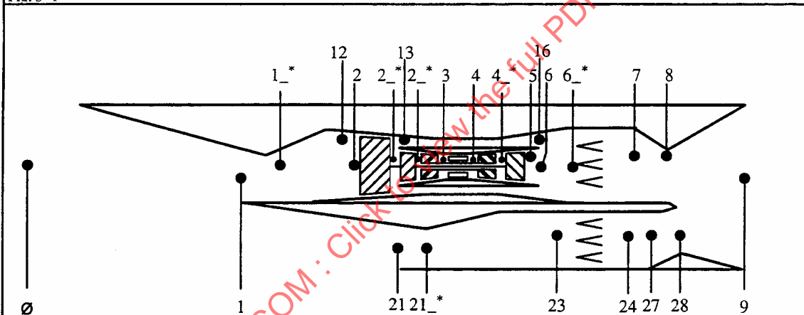
OVER/UNDER TURBORAMJET
