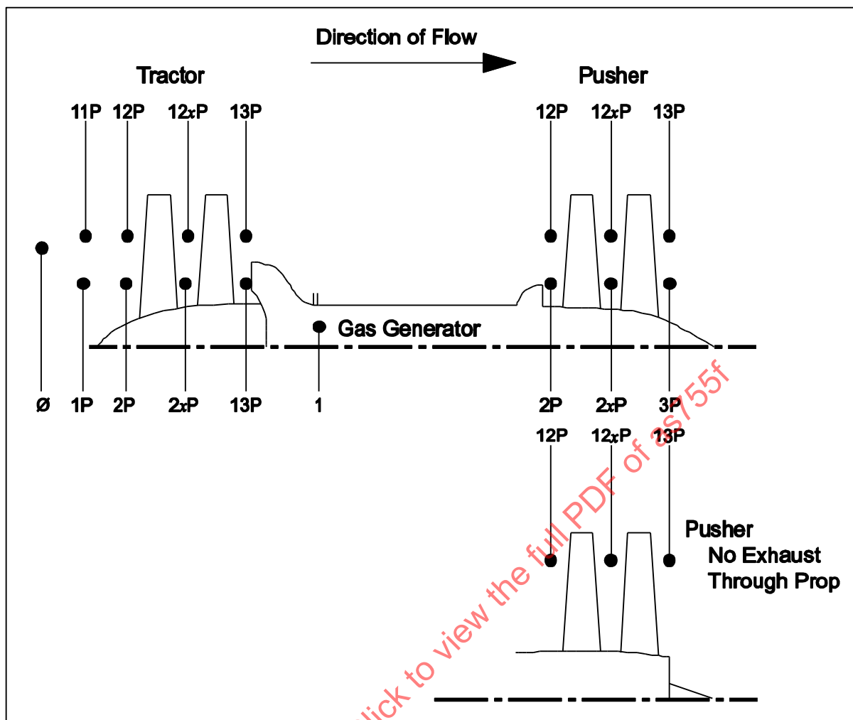
Figure 2 - Propeller/propfan/UDF/ultra-bypass/ultra-high bypass station designations (reference Section 3)
