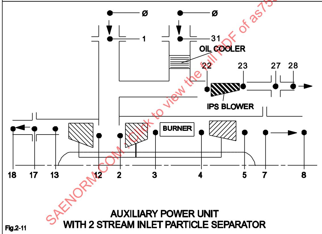
Figure 3 - Examples of station designation for gas turbine engines (reference Section 3) (continued)
