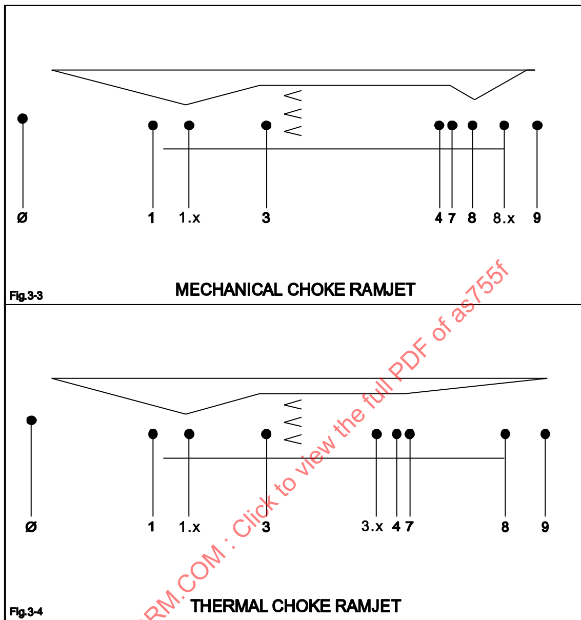
Figure 4 - Examples of station designation for other airbreathing propulsion systems (reference Section 3) (continued)
