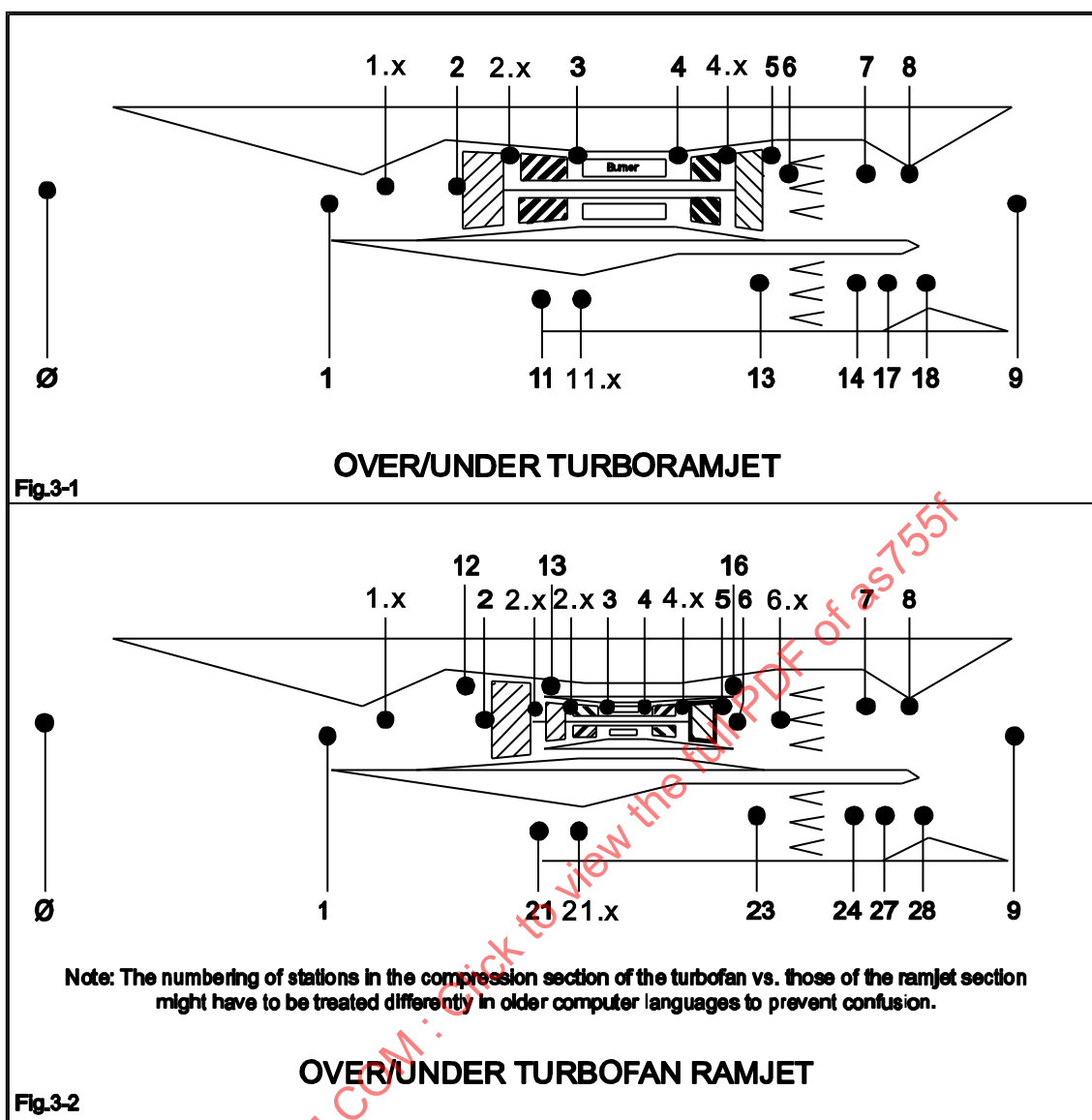
Figure 4 - Examples of station designation for other airbreathing propulsion systems (reference Section 3)
