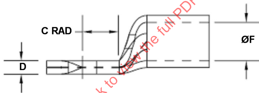
FIGURE 2 - TERMINALS FOR WIRE SIZE 12 THRU 0000 (NO WIRE INSULATION GRIP)
